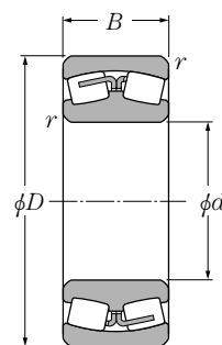
圆柱孔
