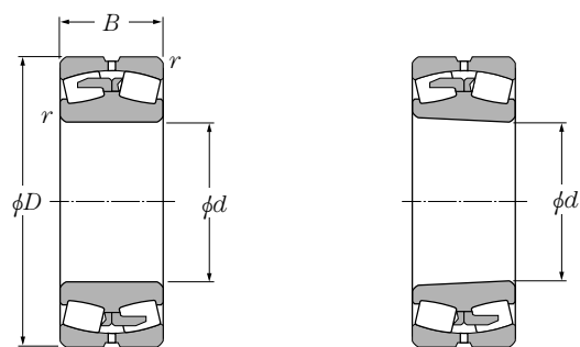
圆柱孔
